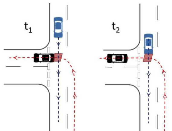
Figure 5.4: Illustration of two moments in time used in the calculation of PET when one vehicle turns left in front of an oncoming vehicle with the right of way. The red rhombus is the encroachment zone. PET = t_2 - t_1 (Figure taken from Bärgman et al., 2015).
